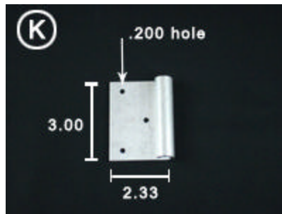
Non Impact Colonial Bifold Hinge
