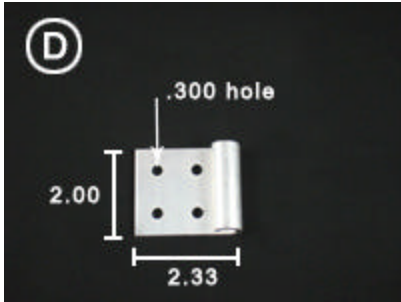
Board and Batten Flat Hinge
