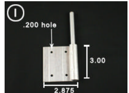
Colonial Flat Hinge with Pin
