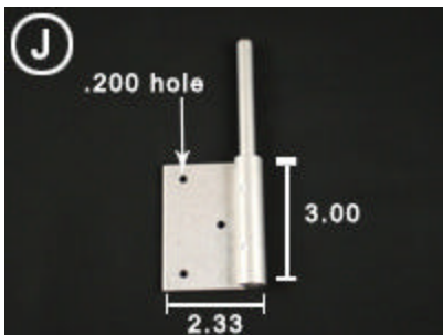
Non Impact Colonial Bifold Flat Hinge with Pin
