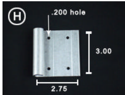
Colonial Flat Hinge
