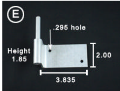
Board and Batten Wall Mount Hinge
