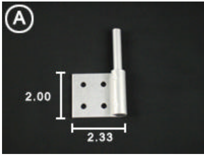
Board and Batten Colonial Hinge with Pin
