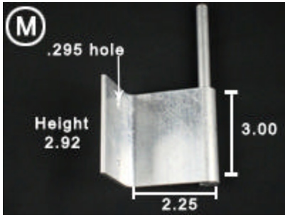
Colonial Double Wall Mount Hinge
